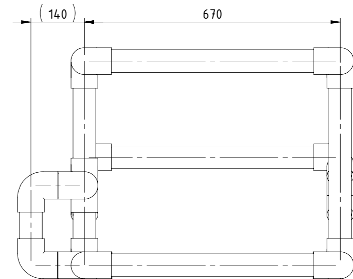
SIDE ELEVATION
