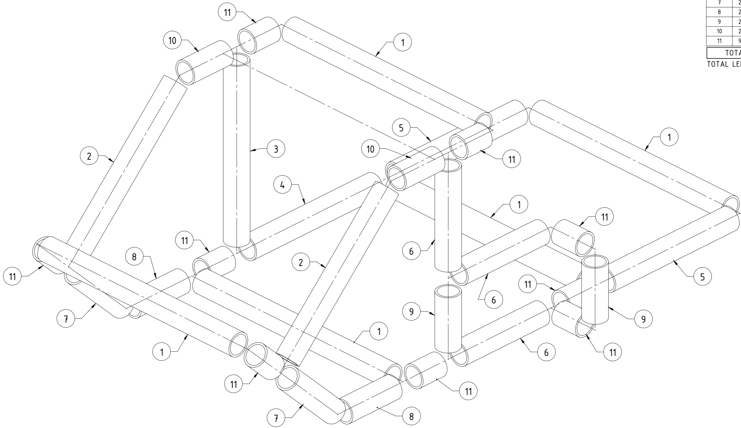
ISOMETRIC NTS
